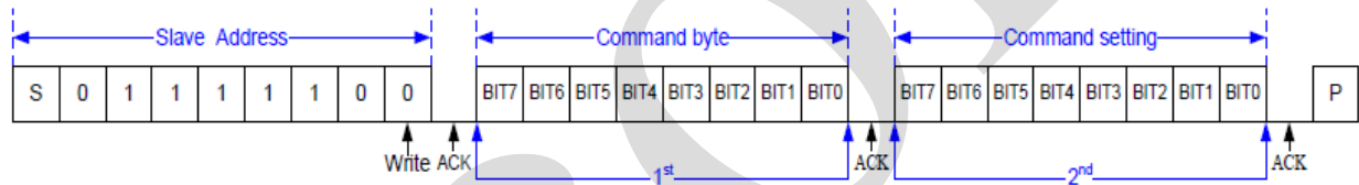
Command Byte Write Operation
