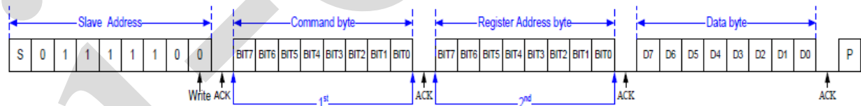
Display RAM Single Data Byte Write Operation
