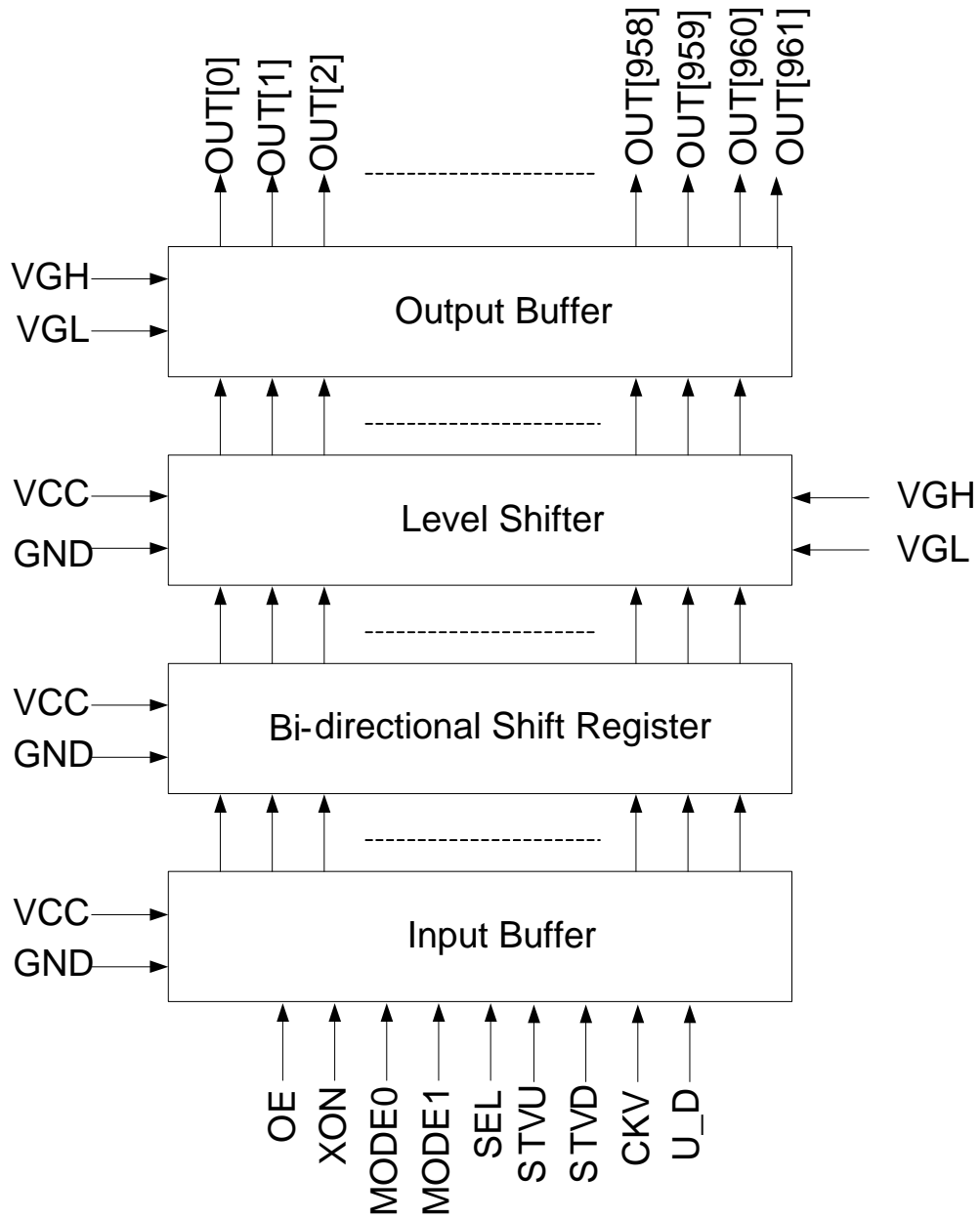
Figure 2. Block Diagram
