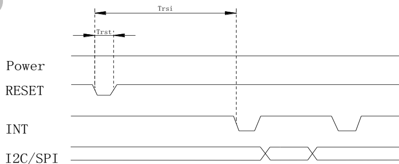
Figure 3-10 Reset Sequence
