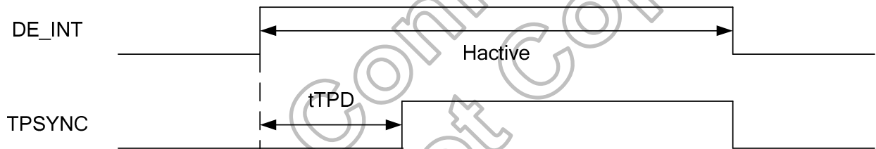
Figure 9.3: TPSYNC timing adjustment
