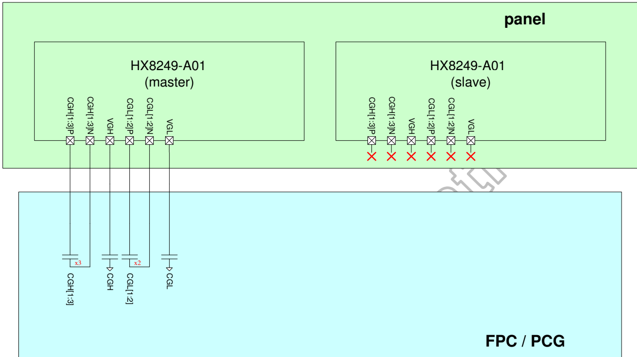
Figure 5.12: Cascade design for charge pumps
