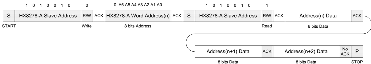
Figure 6.26: I2C format
