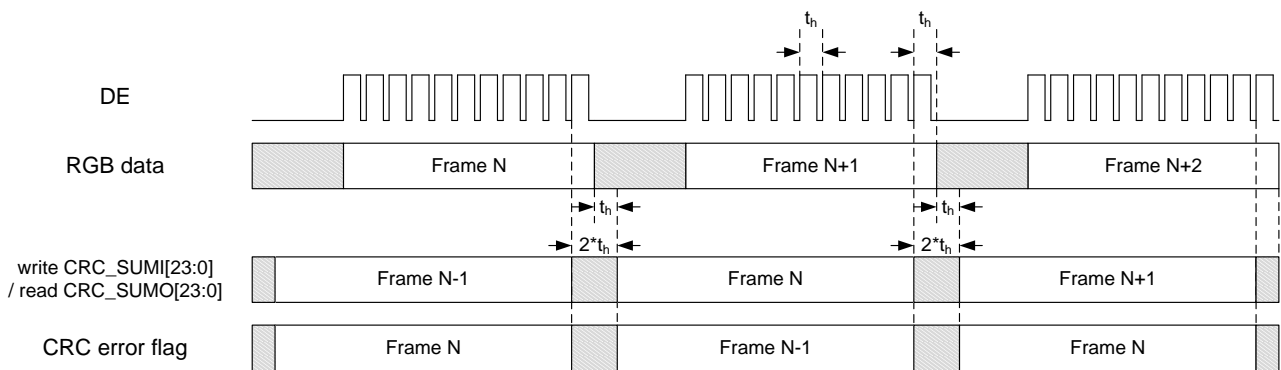
Figure 6.13: CRC timing
