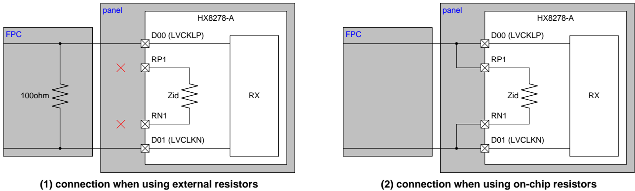
Figure 4.4: Connection of termination resistors
