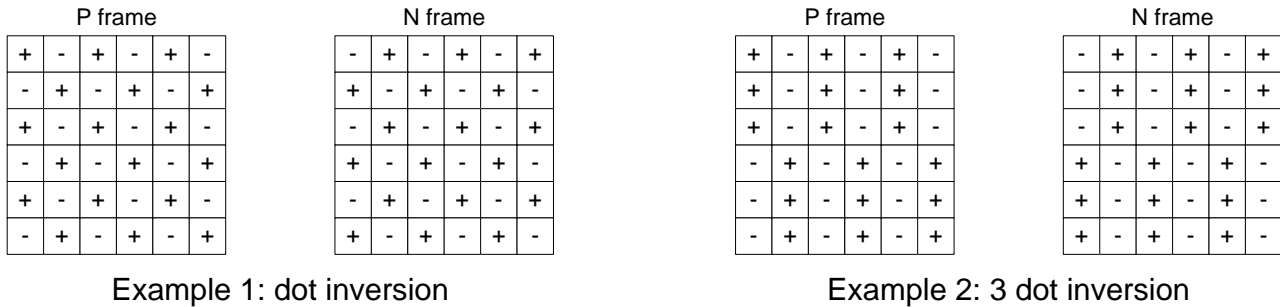
Figure 6.18: Definition of frame polarity
