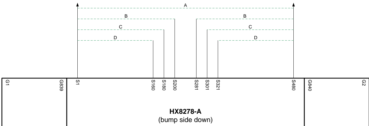
Figure 5.2: Valid source output
