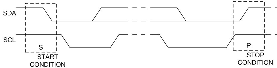
Figure 4.7: I²C START/STOP
