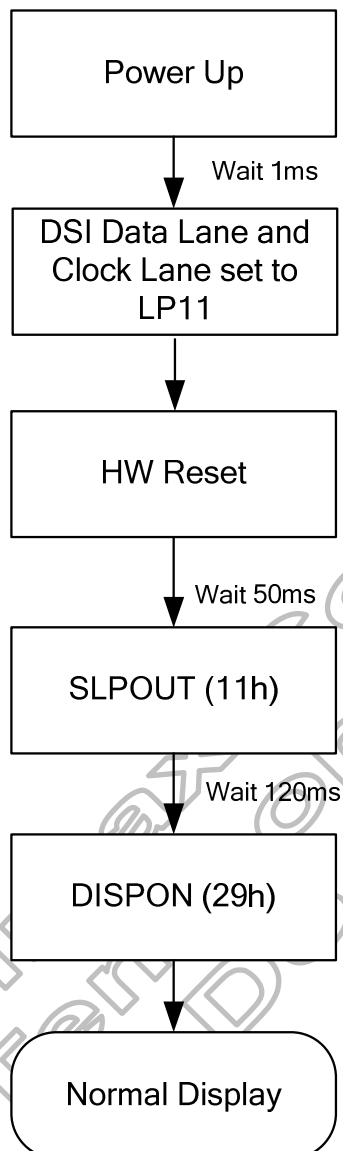
Figure 5.29: Power on/off sequence
