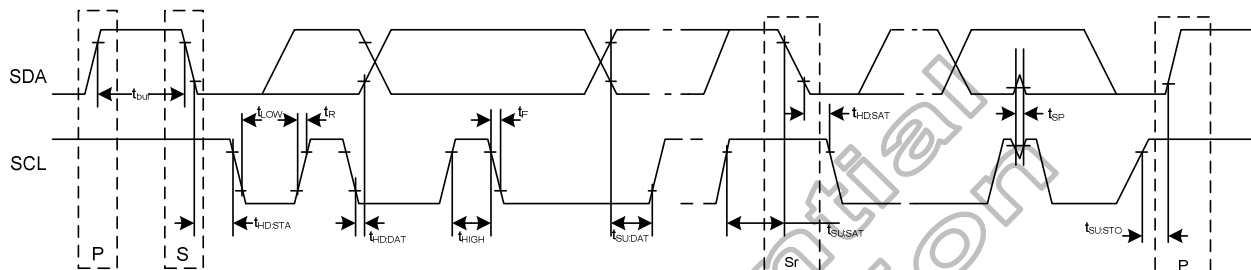
Figure 8.1: I2C timing
