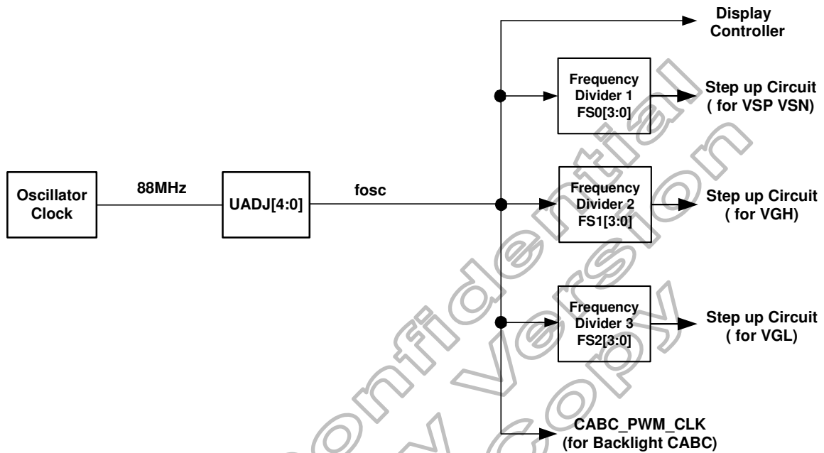
Figure 5.8: OSC aritecture
