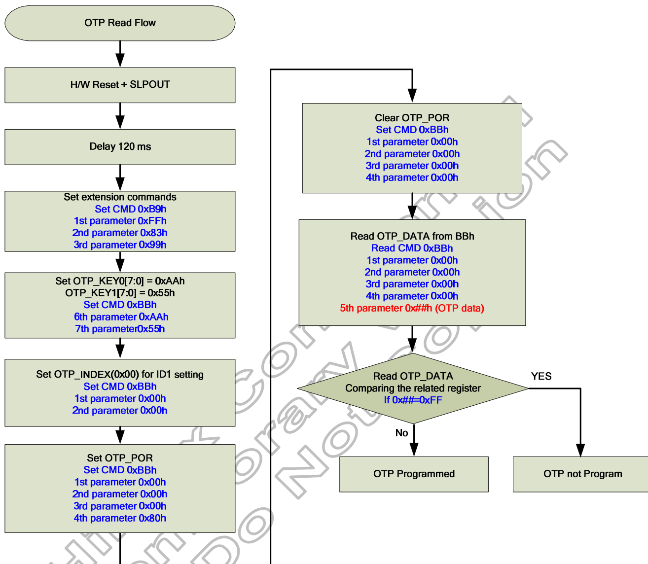
Figure 5.51: OTP read sequence flow of Index 00h
