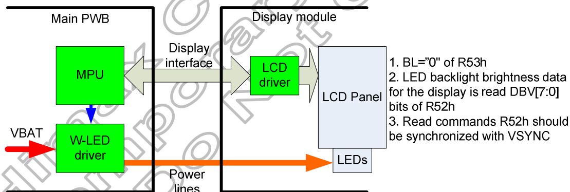
Figure 5.41: Module architecture
