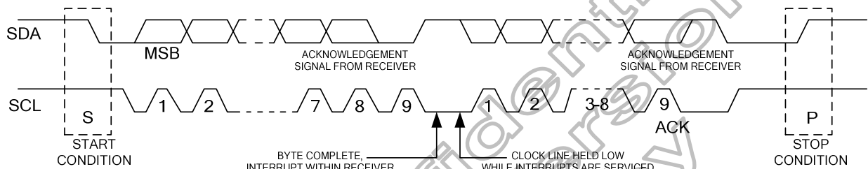
Figure 4.8: I²C data transfer
