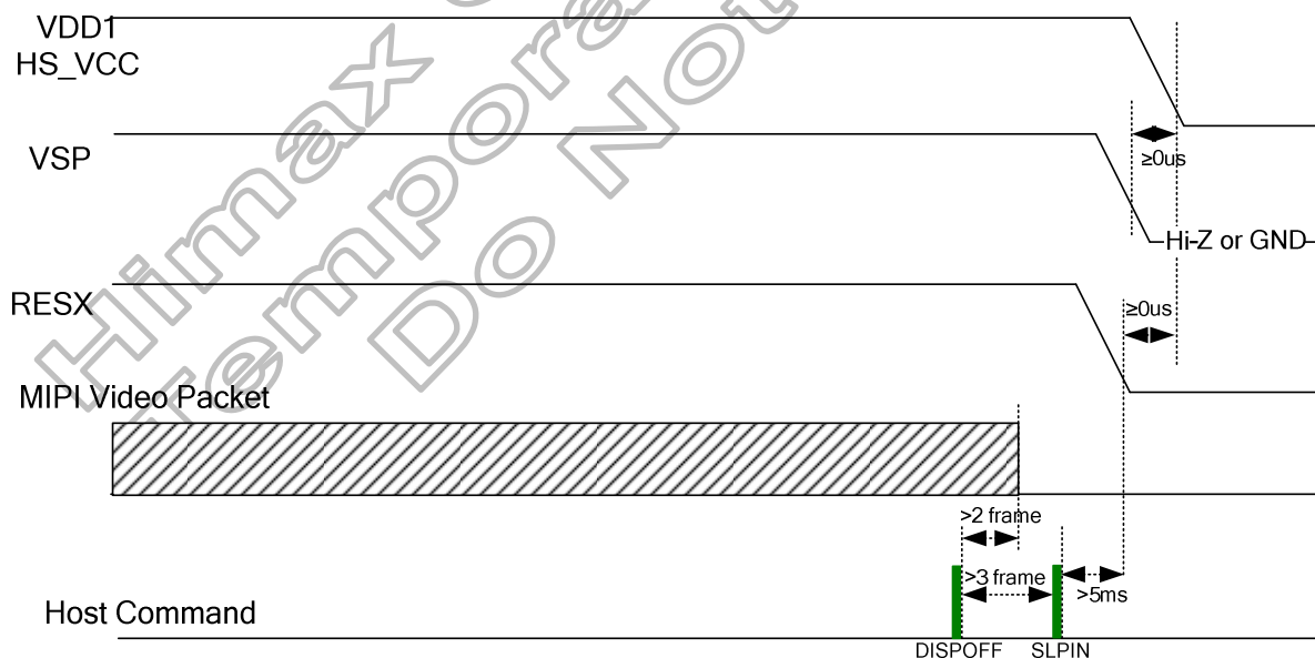
Figure 5.33: VSP/VDD1 input power off sequence (PCCS[2:0] =010)
