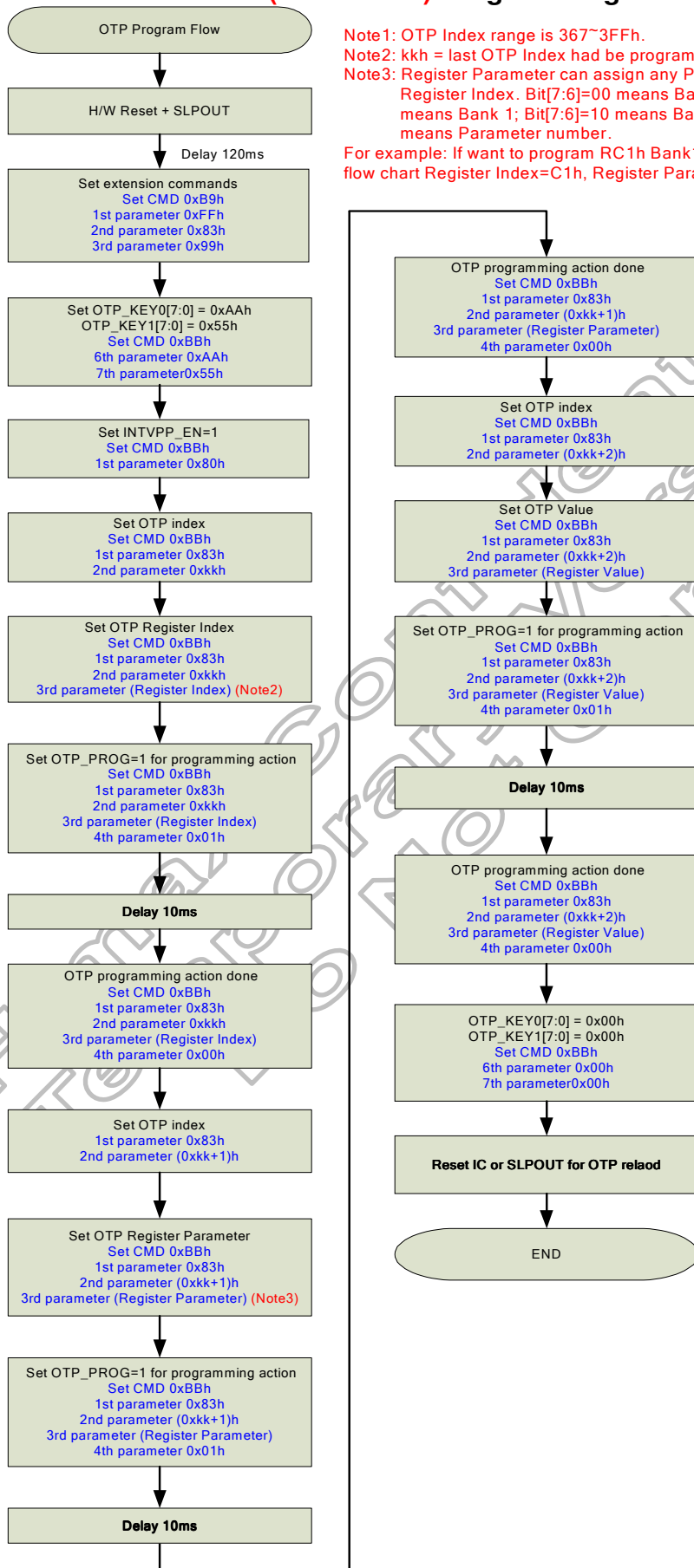
Figure 5.49: Flexible OTP programming sequence
