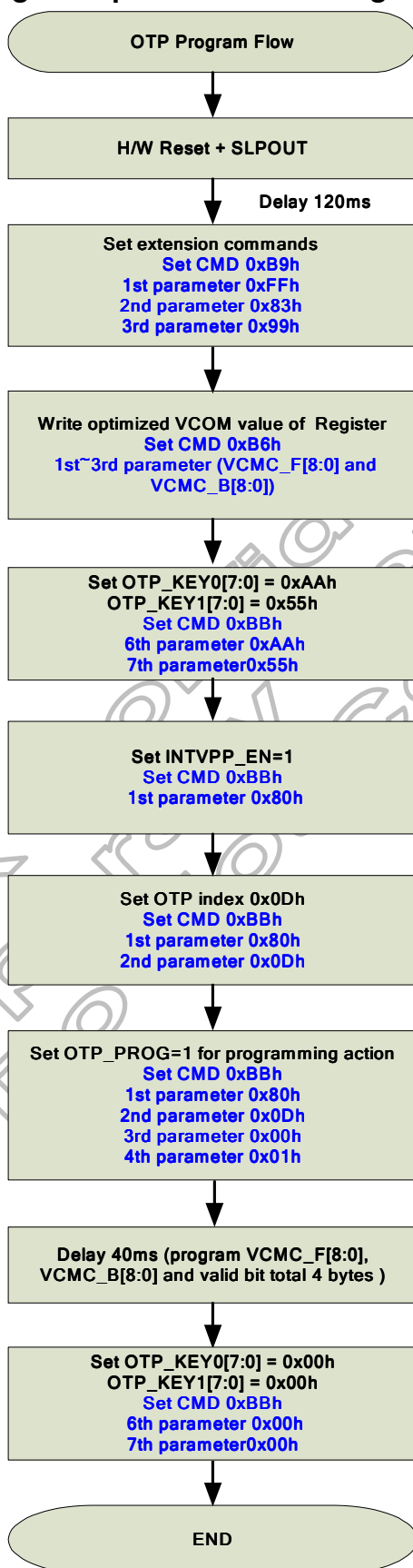
Figure 5.46: OTP programming sequence example 1
