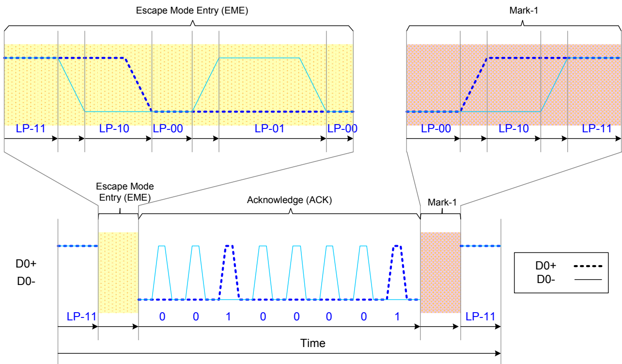
Figure 28 Acknowledge (ACK)
