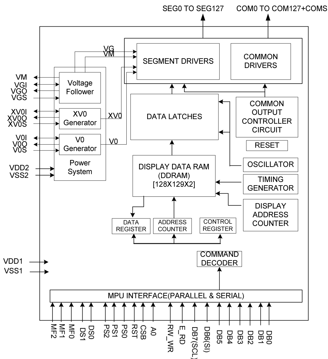
Fig.2 Block diagram
