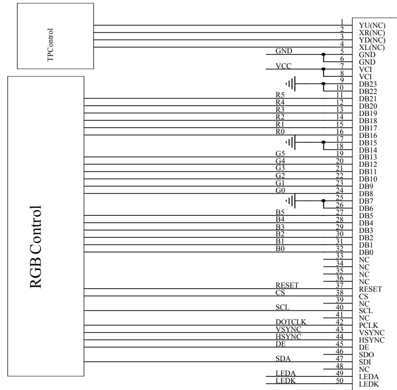
E40RB-FW600-N FPC
