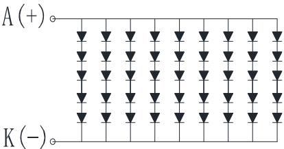
BL CIRCUIT DIAGRAM
