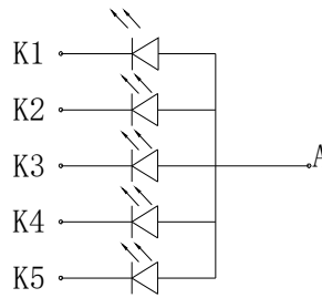
B/L Circuit
