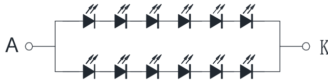
BL CIRCUIT DIAGRAM
