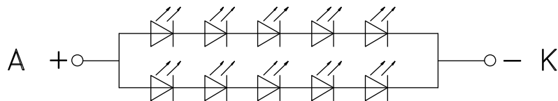
BL CIRCUIT DIAGRAM
