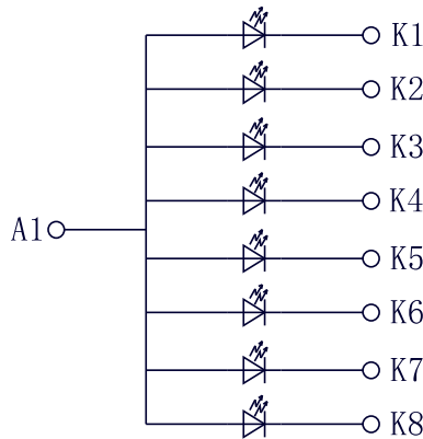
BL CIRCUIT DIAGRAM
