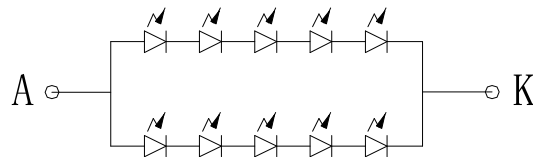
BL CIRCUIT DIAGRAM
