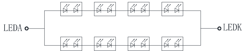
BL CIRCUIT DIAGRAM
