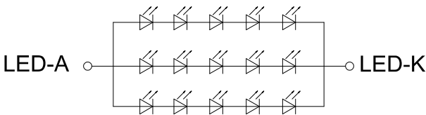
BL CIRCUIT DIAGRAM
