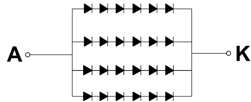
BL CIRCUIT DIAGRAM
