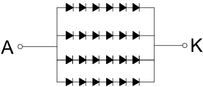
BL CIRCUIT DIAGRAM
