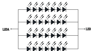
BL CIRCUIT DIAGRAM
