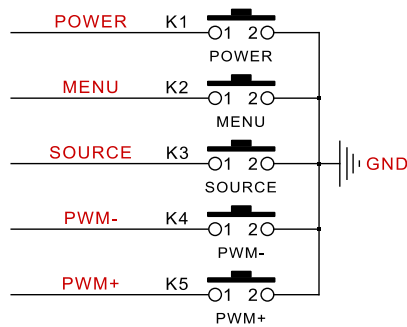
OSD key circuit diagram
