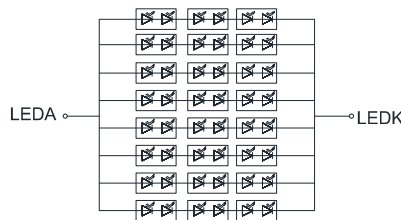
BL CIRCUIT DIAGRAM
