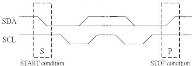
Figure 4 Definition of START and STOP conditions
